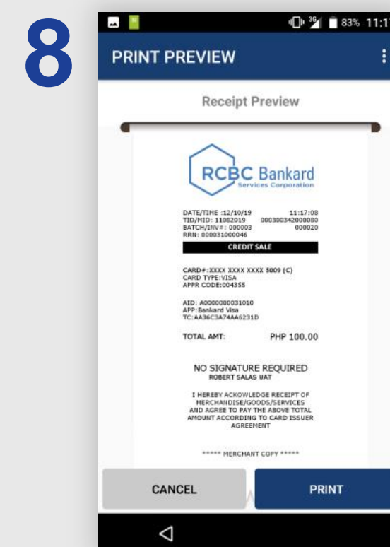
Print Receipt
