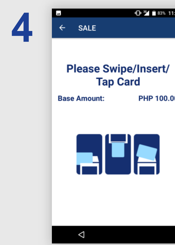
Tap Card
