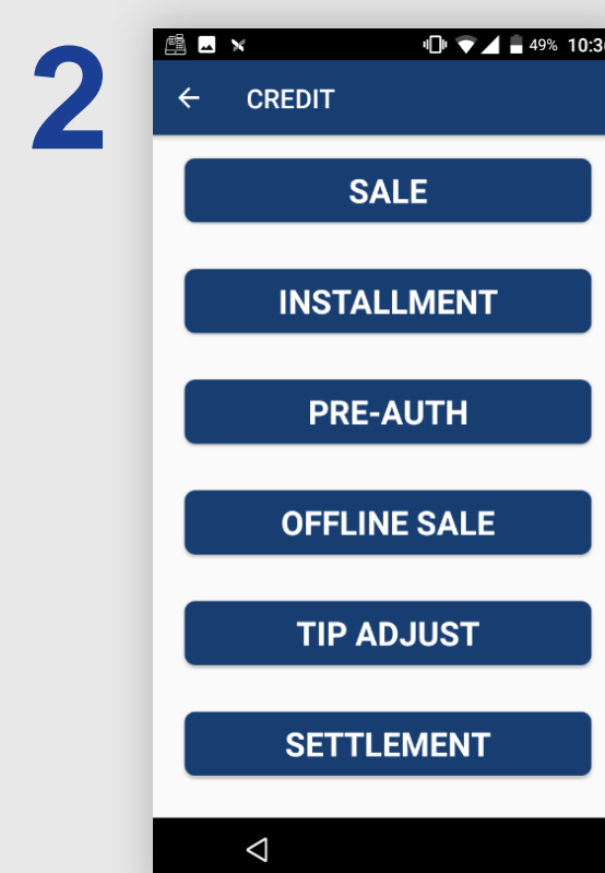
Select Sale
