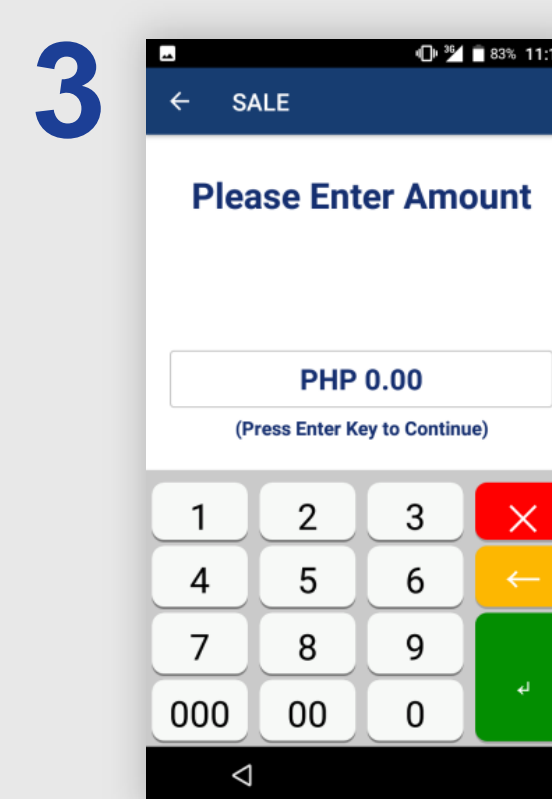
Enter Amount
